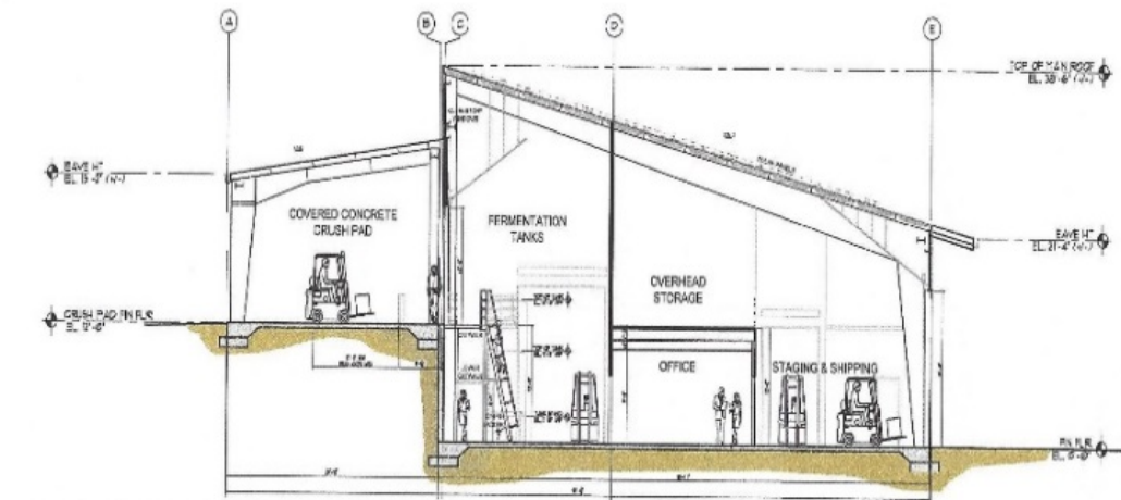
A1 BUILDING SECTION 1/8" = 1'-0"
